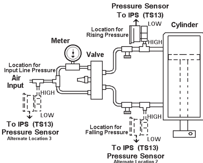
Figure 6-3. IPS System with Differential Pressure Sensor
