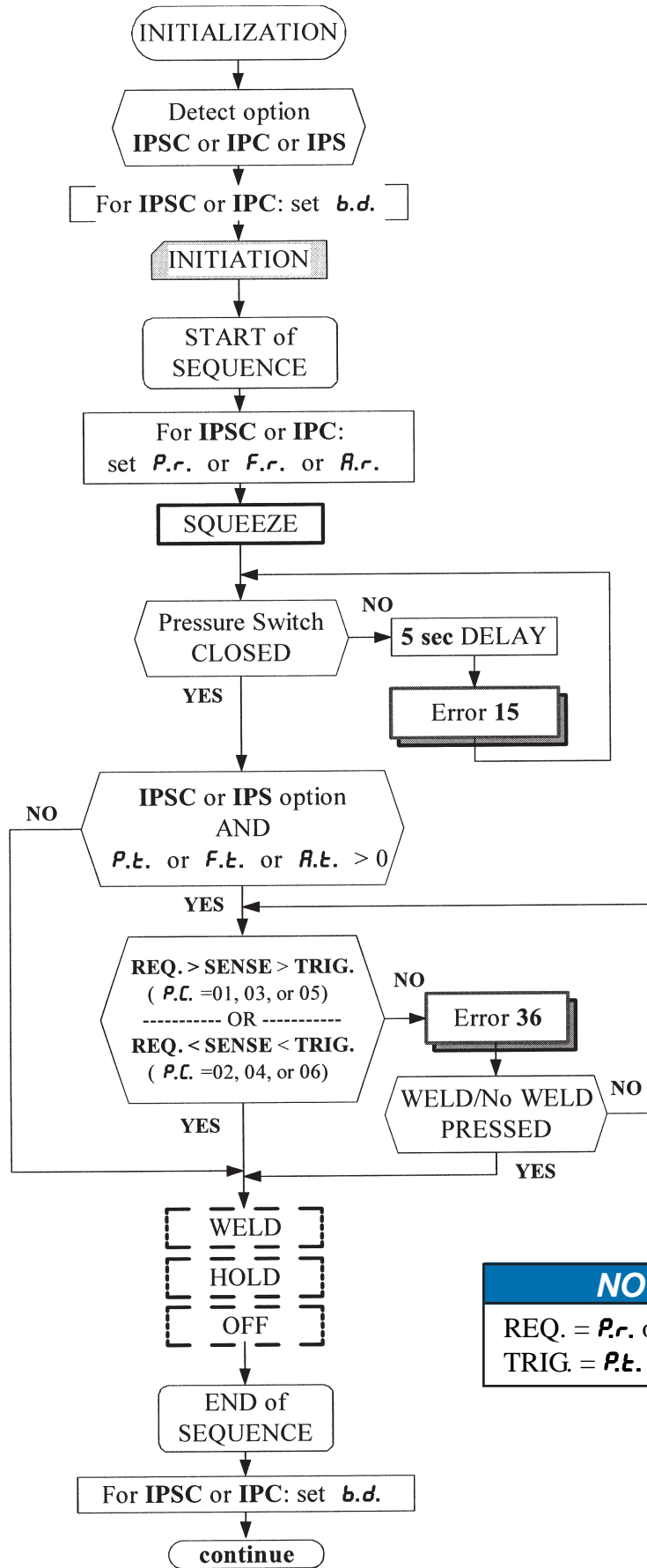
Figure 3-1. Sequence Algorithm
