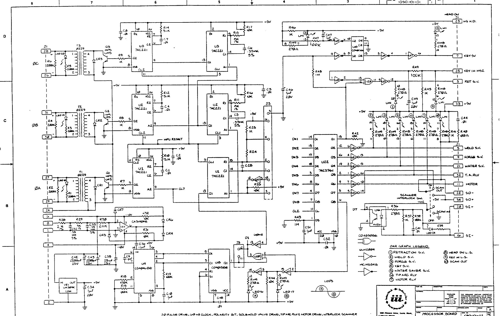
3/2 PULSE DRIVE, 1/40 Hz CLOCK, POLARITY BT, SOLIDSHOLD VALVE DRIVE, TIP ARC RLY & MOTOR DRIVE, INTERLOCK SCANNER
